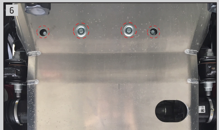
6 In the middle connect bracket (B) to the plate (A) using hex bolt (E), spring washer (I), and washer (D)
