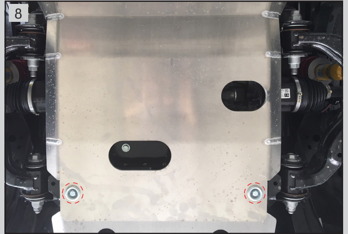
Connect the plate to original screwing using hex bolt (F), spring washer (I), pocket washer (D). Tighten all 6 bolts of the skid plate
