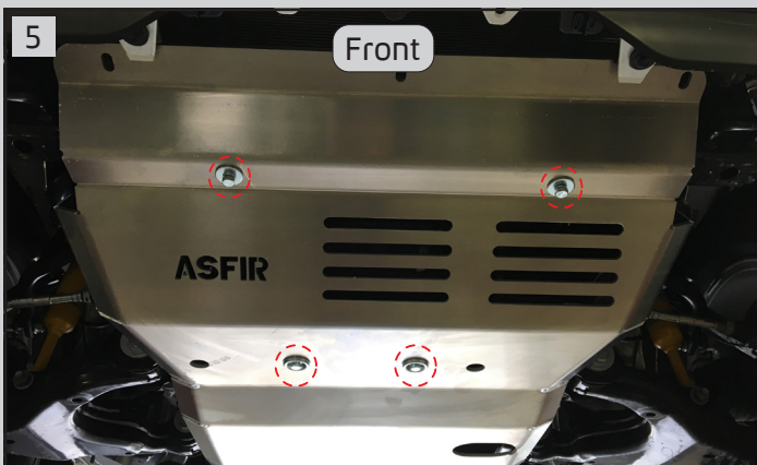
5 In the front, connect plate (A) to original screwing using hex bolt (E), spring washer (I) and washer (G).
