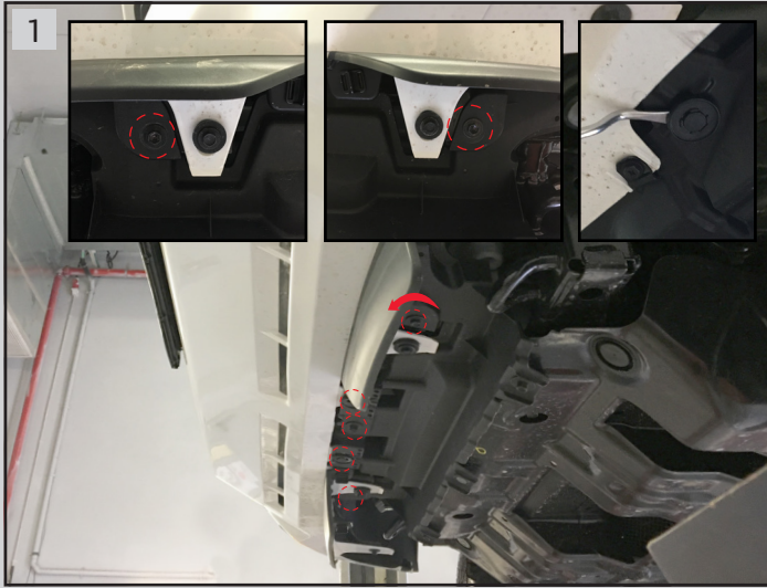
1 Remove the 3 bolts and 2 clips
