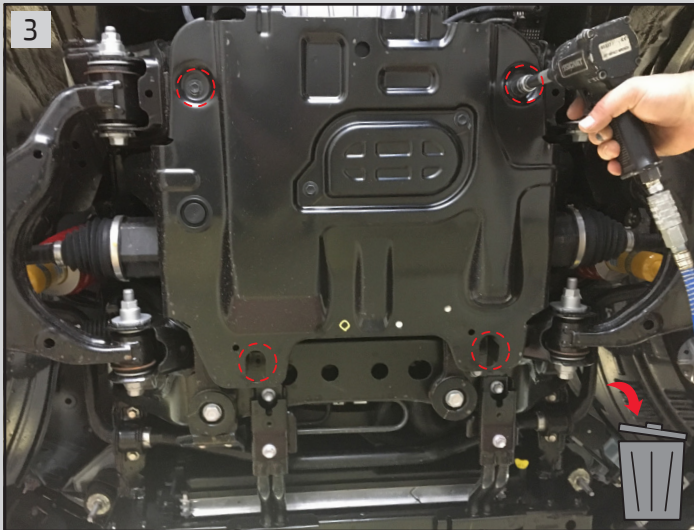
3 Remove 4 bolts and dispose the original plate
